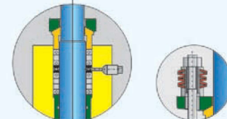
Stem seal
