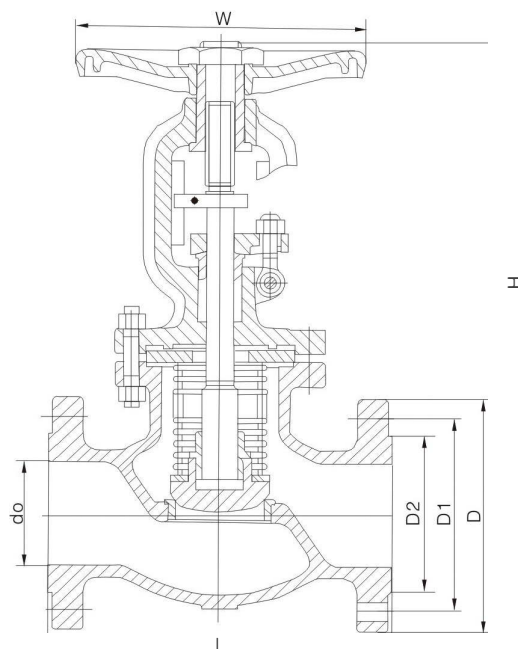
Main External and Connecting Dimensions
